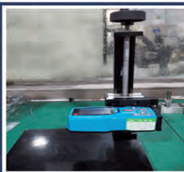
粗糙仪 Roughness Tester
